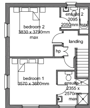
First Floor Plan - 2 bed option
