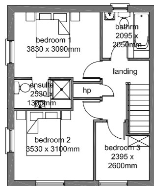
First Floor Plan - 3 bed option
