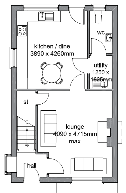
Ground Floor Plan 939 sq ft
