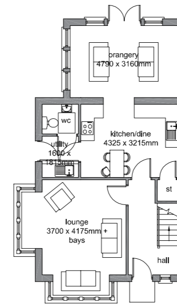
Ground Floor Plan 1/200 1119 sqft
