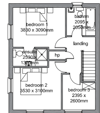
First Floor Plan 1/200 - 3 bed option
