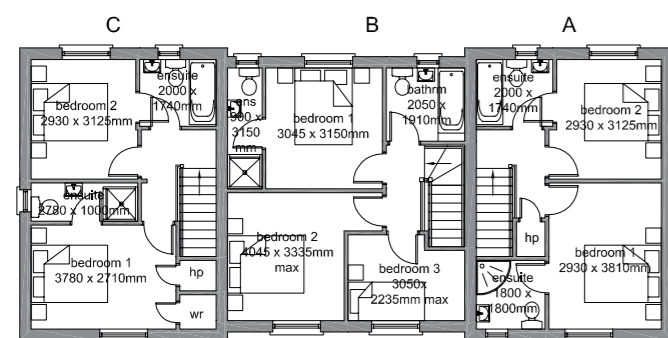
First Floor Plan (2 bed option)
