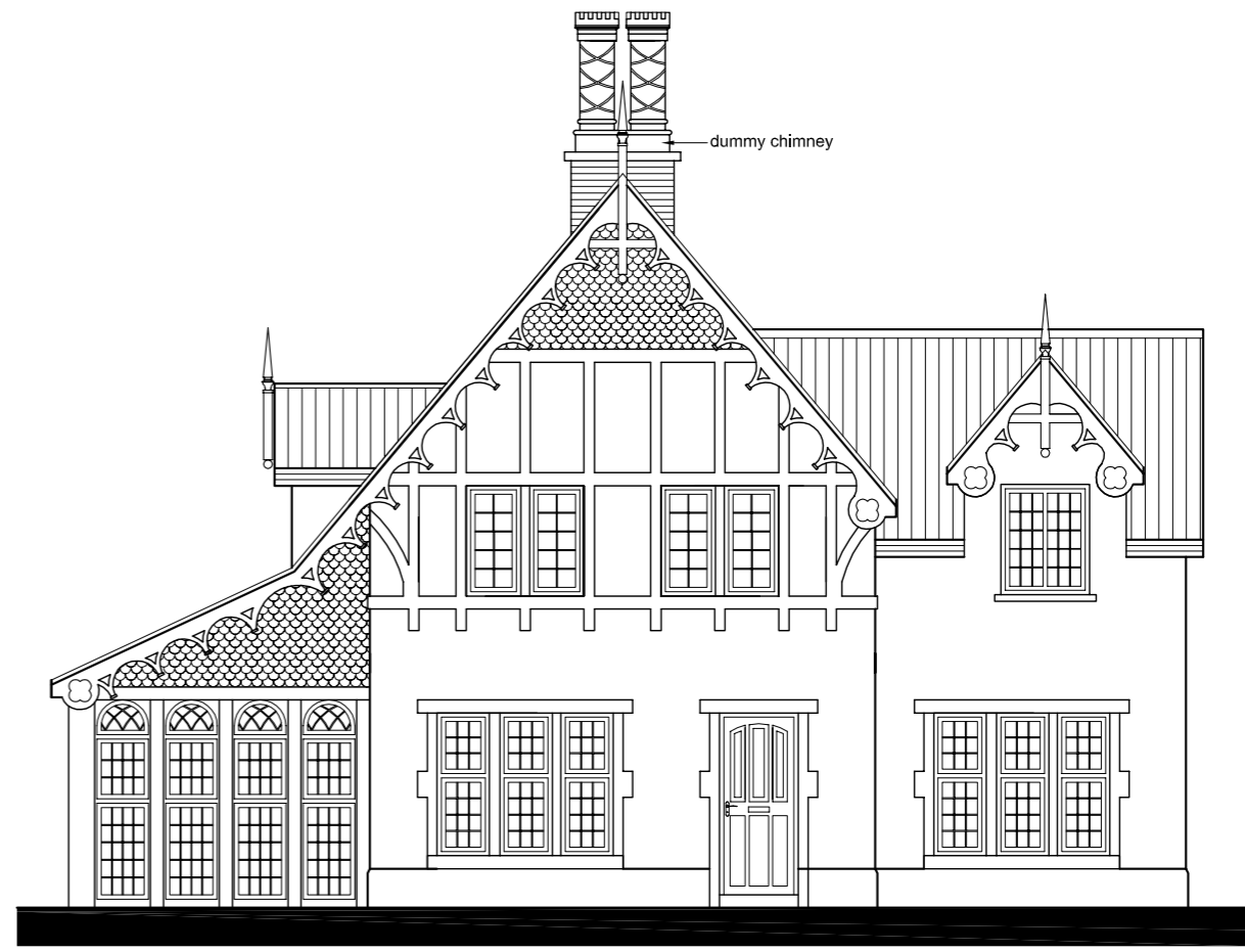
Front Elevation 1/100
