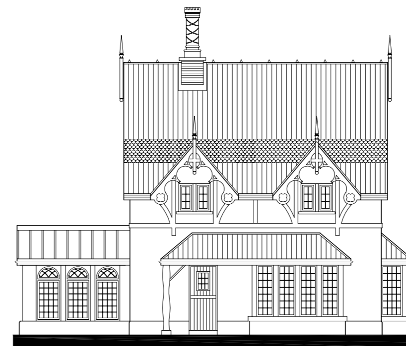
Side Elevation 1/100
