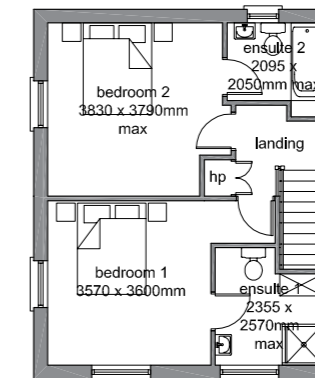
First Floor Plan 1/200 - 2 bed option
